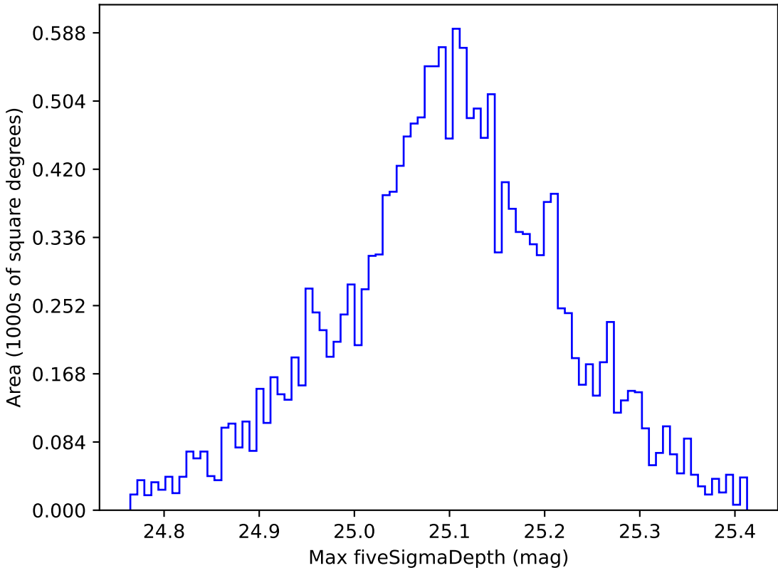
weather_cloudso30v3.4_10yrs WFD all bands: Max fiveSigmaDepth
