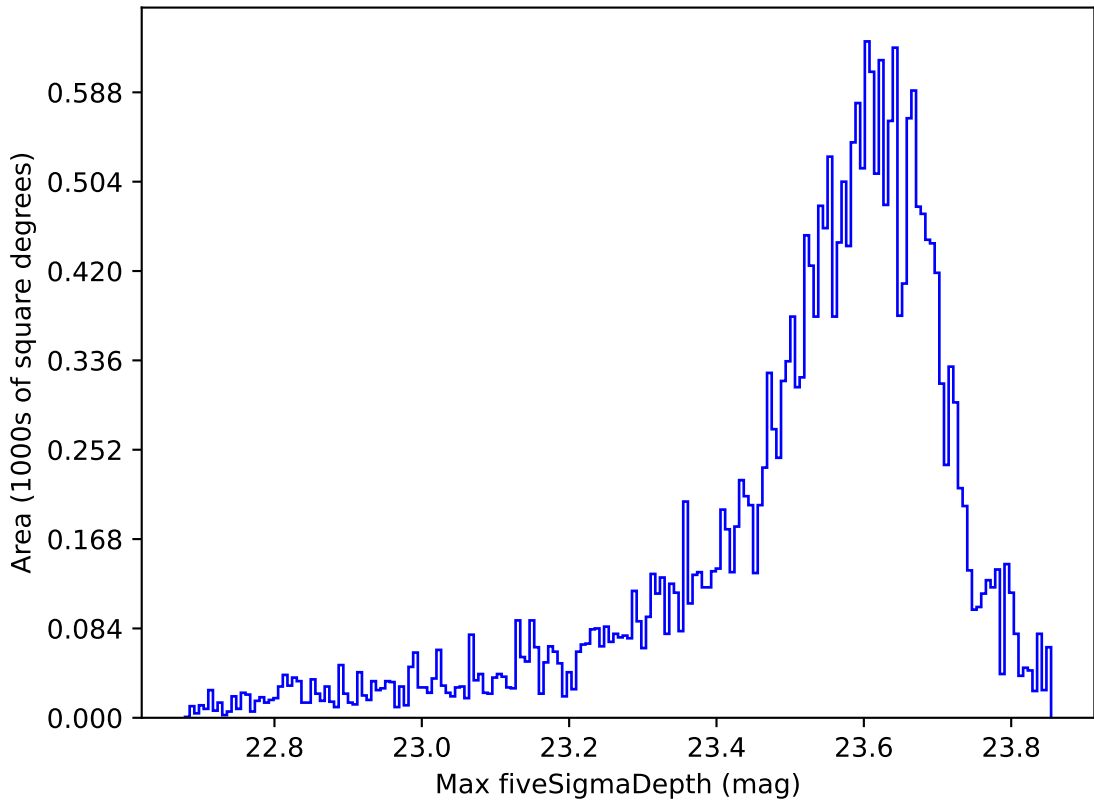
weather_cloudso30v3.4_10yrs All sky z band: Max fiveSigmaDepth
