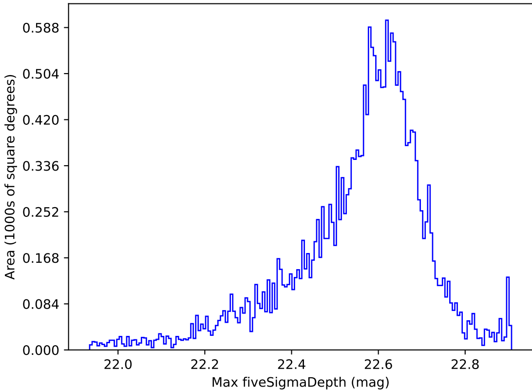
weather_cloudso30v3.4_10yrs All sky y band: Max fiveSigmaDepth
