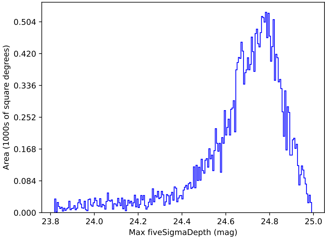
weather_cloudso30v3.4_10yrs All sky r band: Max fiveSigmaDepth
