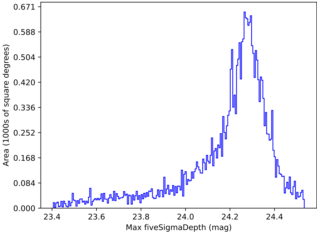
weather_cloudso30v3.4_10yrs All sky i band: Max fiveSigmaDepth
