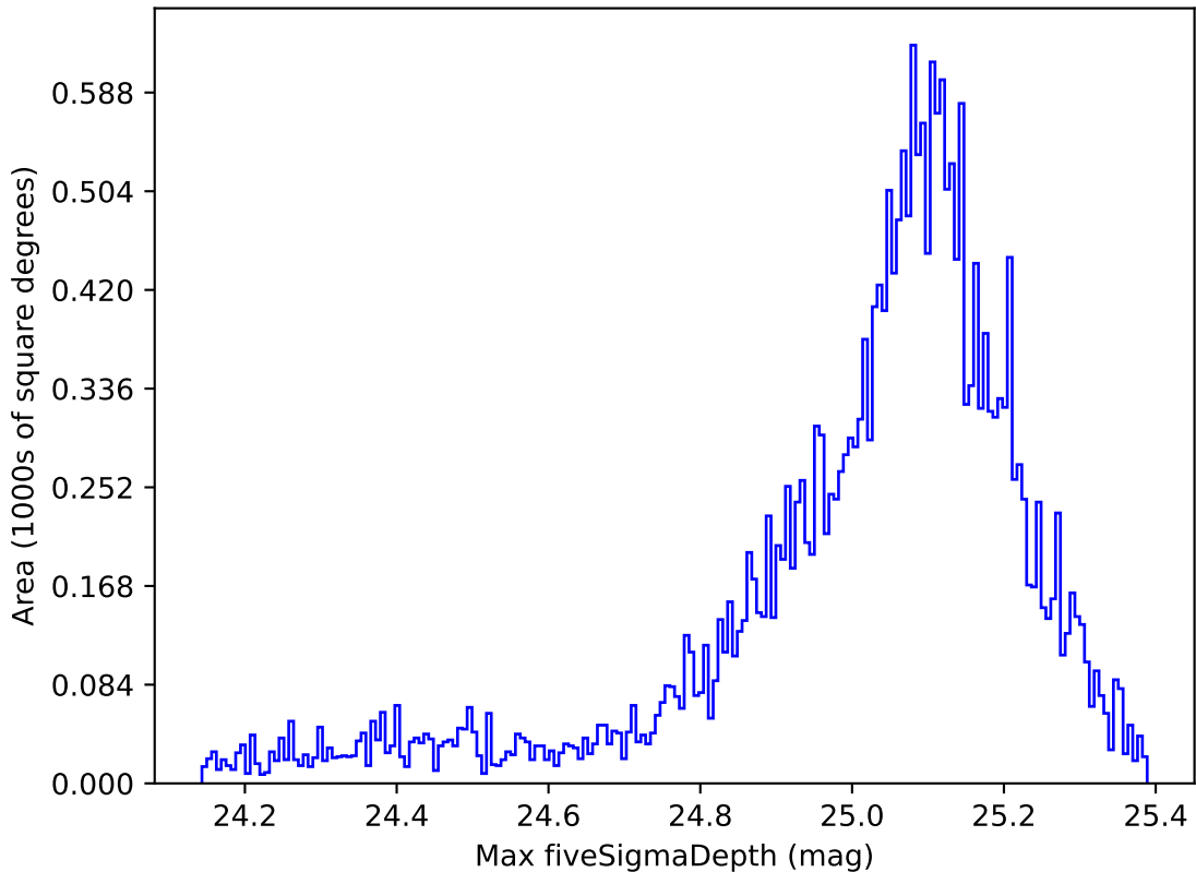
weather_cloudso30v3.4_10yrs All sky g band: Max fiveSigmaDepth
