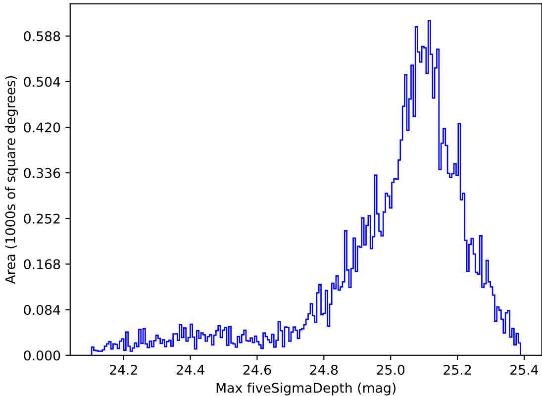
weather_cloudso30v3.4_10yrs All sky all bands: Max fiveSigmaDepth
