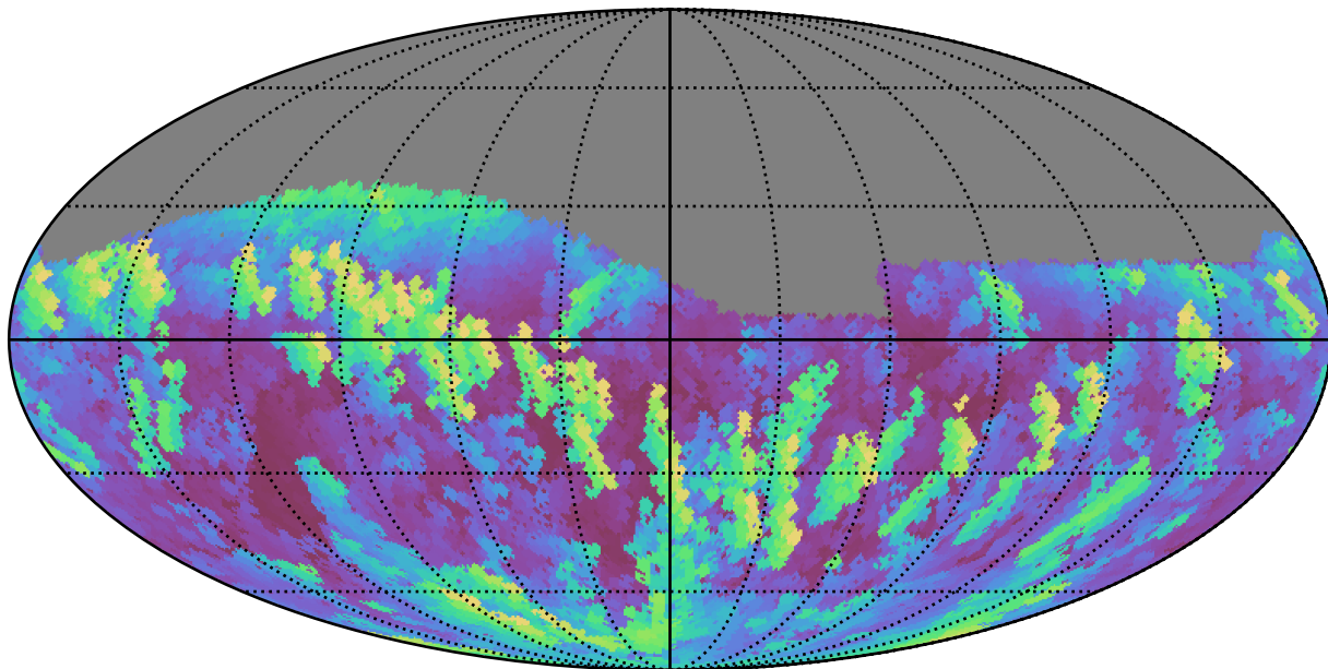
weather_cloudso30v3.4_10yrs Yr 1 z band: Max airmass
