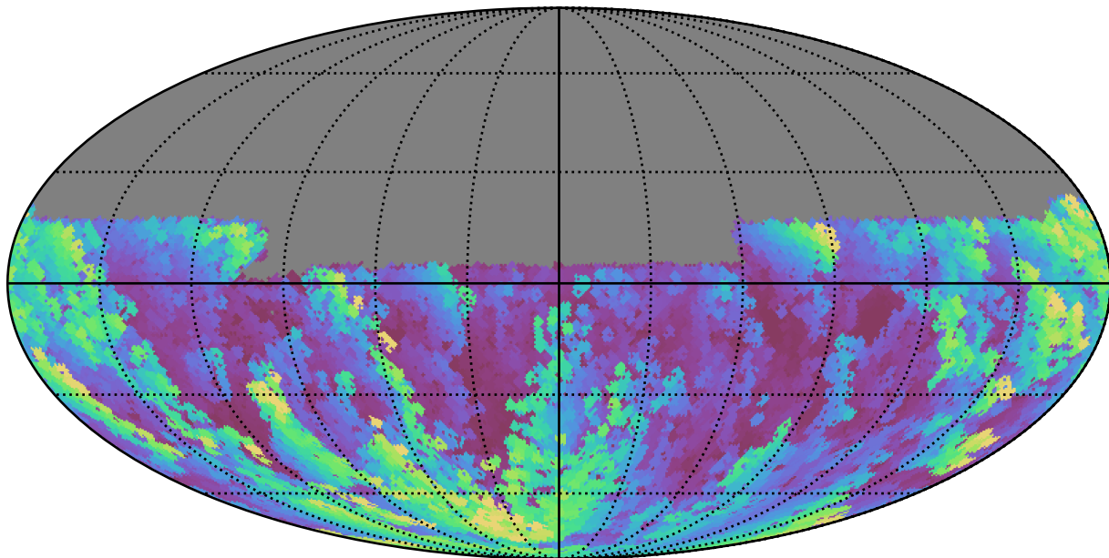
weather_cloudso30v3.4_10yrs Yr 1 y band: Max airmass
