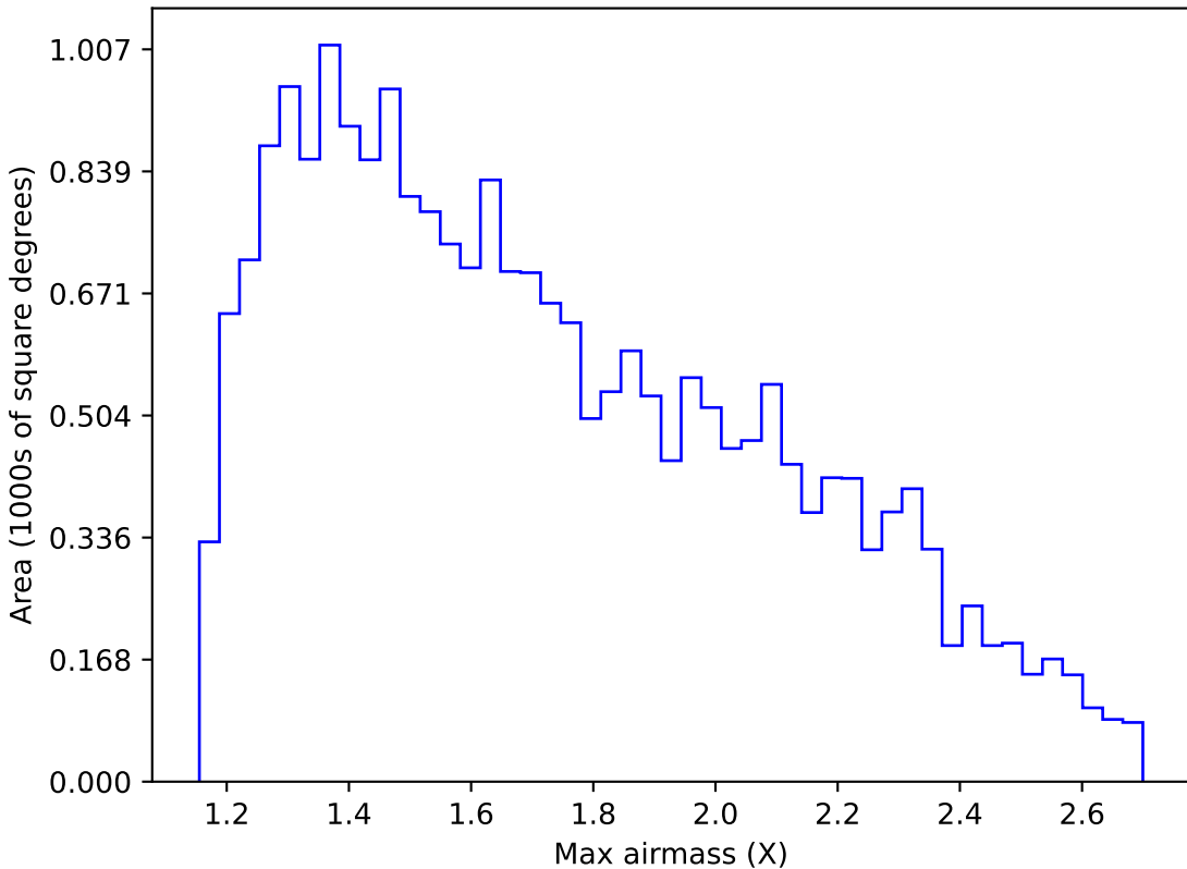
weather_cloudso30v3.4_10yrs Yr 1 y band: Max airmass
