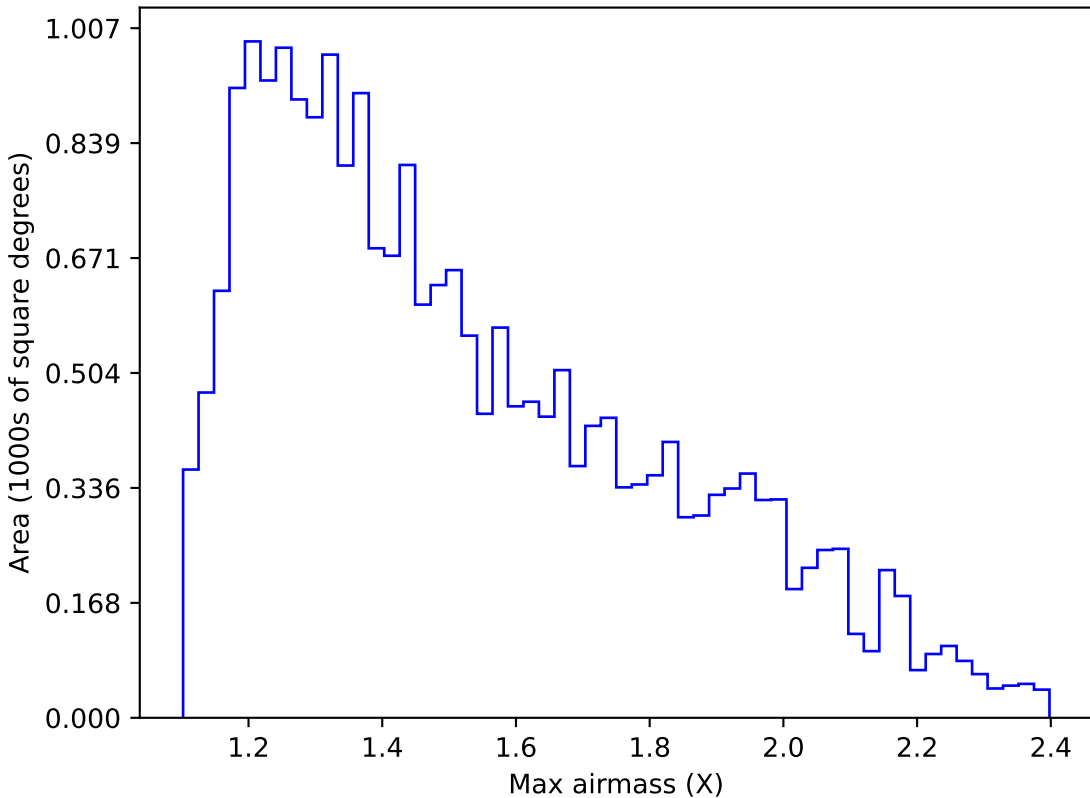
weather_cloudso30v3.4_10yrs Yr 1 u band: Max airmass
