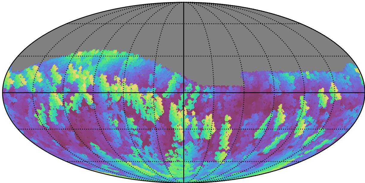
weather_cloudso30v3.4_10yrs Yr 1 i band: Max airmass
