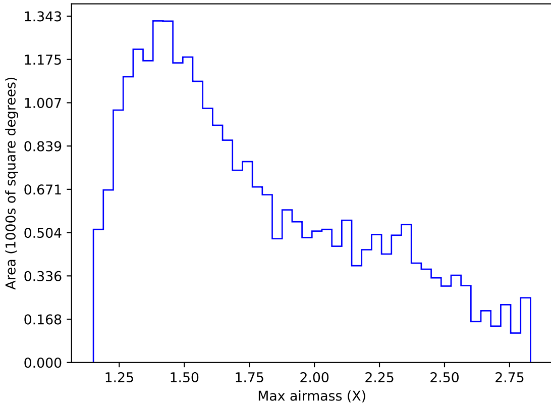
weather_cloudso30v3.4_10yrs Yr 1 i band: Max airmass
