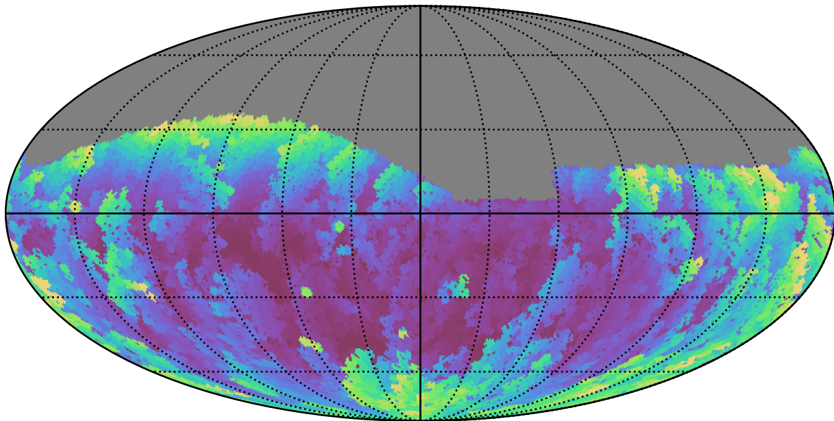
weather_cloudso30v3.4_10yrs Yr 1 g band: Max airmass
