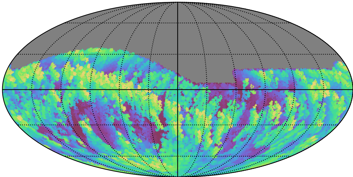
weather_cloudso30v3.4_10yrs Yr 1 all bands: Max airmass
