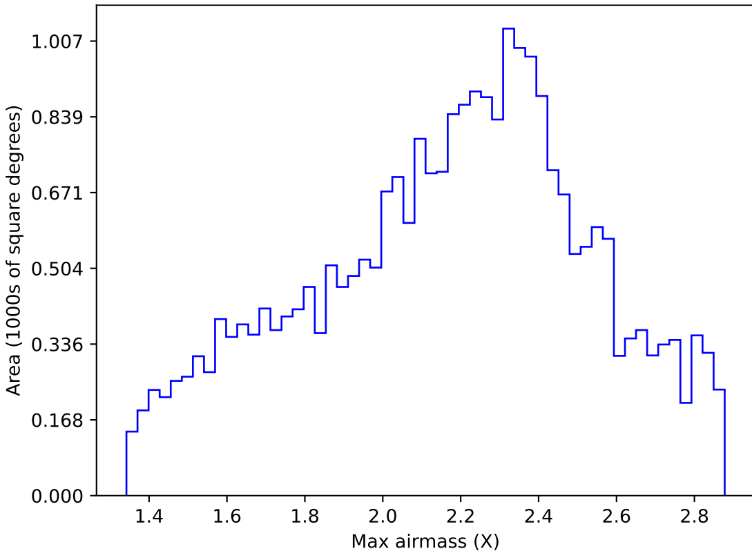
weather_cloudso30v3.4_10yrs Yr 1 all bands: Max airmass
