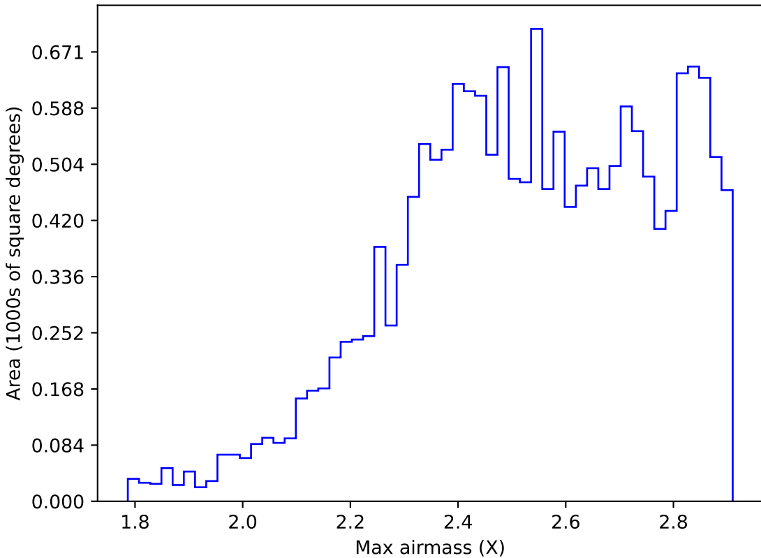
weather_cloudso30v3.4_10yrs WFD z band: Max airmass
