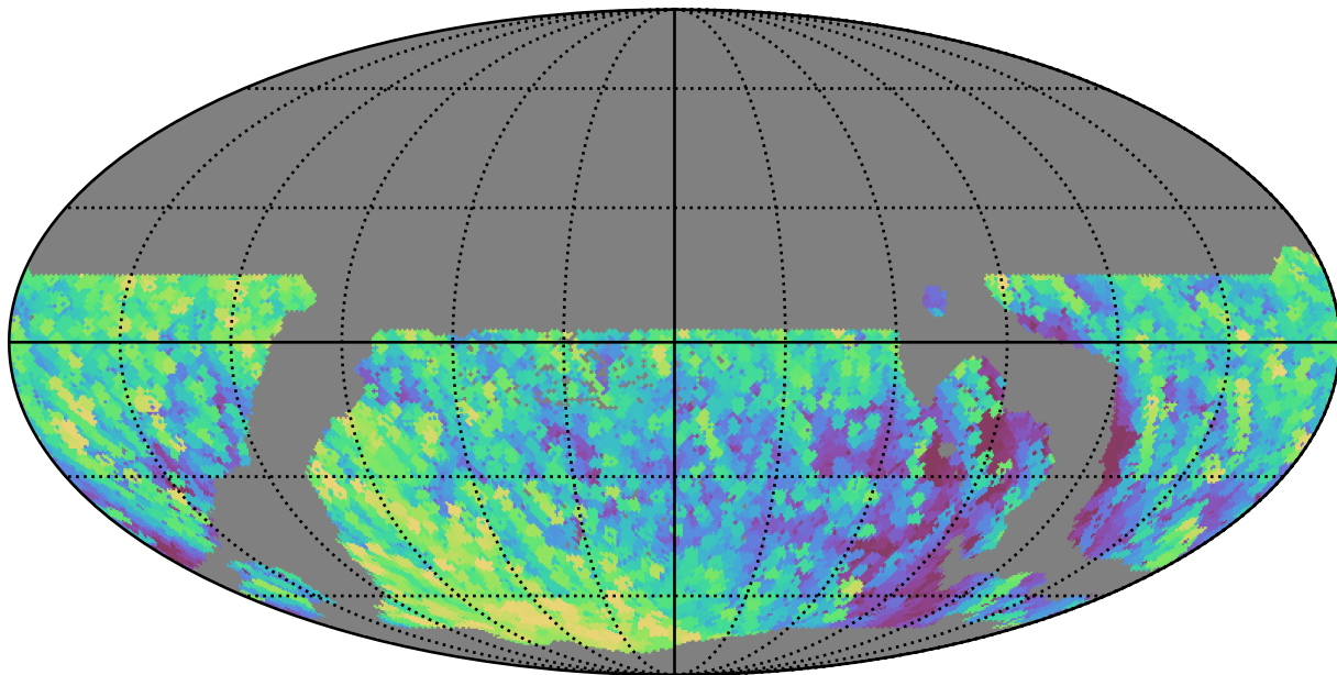
weather_cloudso30v3.4_10yrs WFD y band: Max airmass
