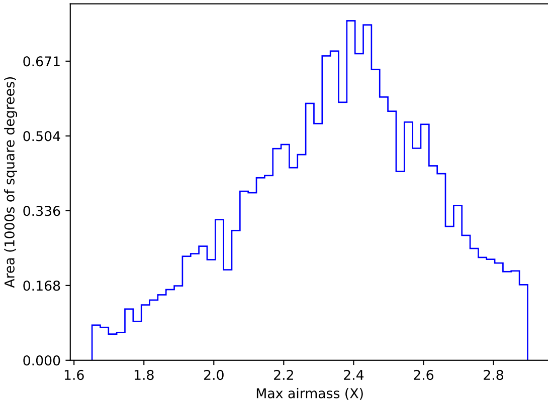
weather_cloudso30v3.4_10yrs WFD y band: Max airmass
