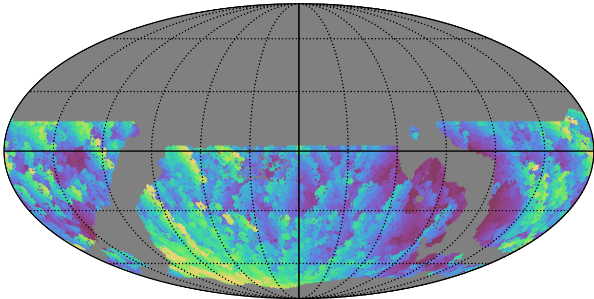
weather_cloudso30v3.4_10yrs WFD u band: Max airmass
