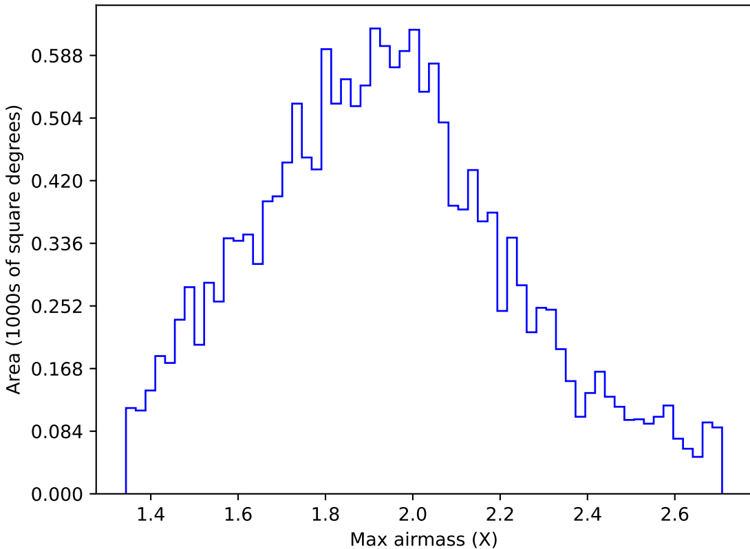
weather_cloudso30v3.4_10yrs WFD u band: Max airmass
