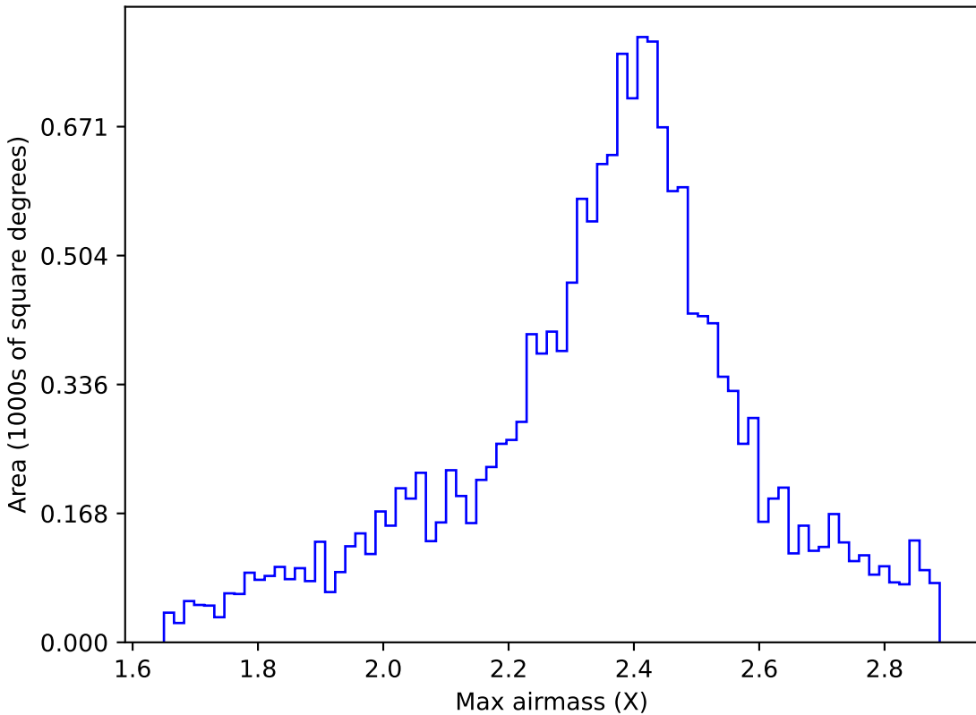
weather_cloudso30v3.4_10yrs WFD r band: Max airmass
