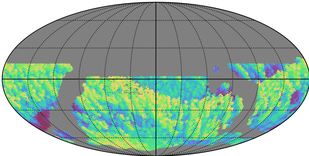
weather_cloudso30v3.4_10yrs WFD i band: Max airmass
