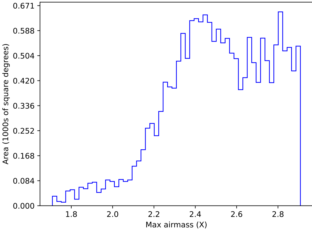
weather_cloudso30v3.4_10yrs WFD i band: Max airmass
