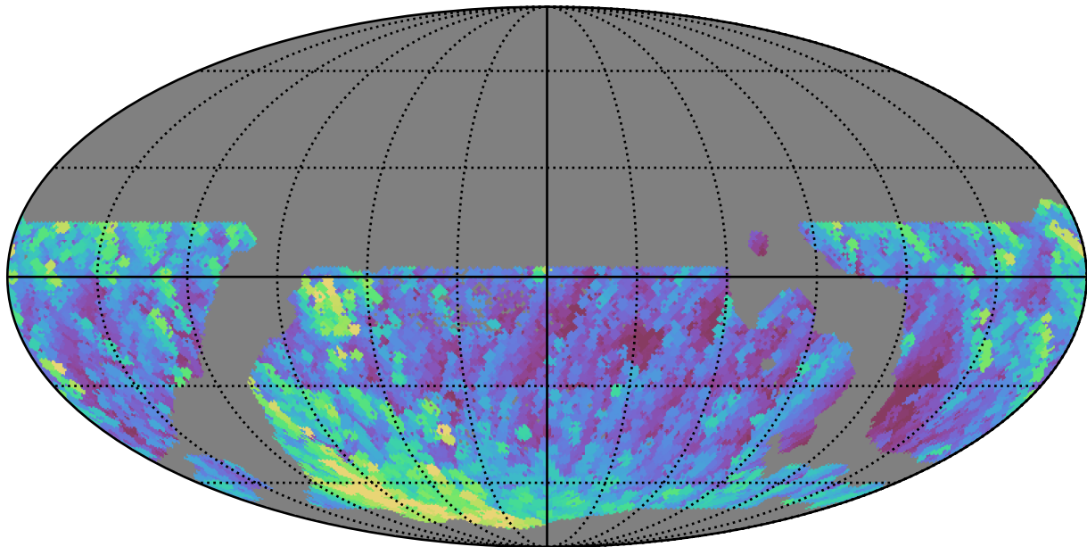
weather_cloudso30v3.4_10yrs WFD g band: Max airmass
