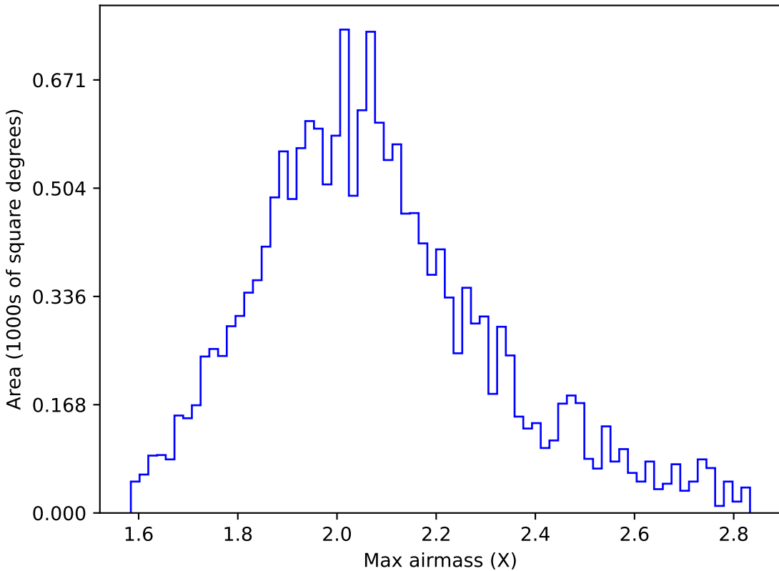
weather_cloudso30v3.4_10yrs WFD g band: Max airmass
