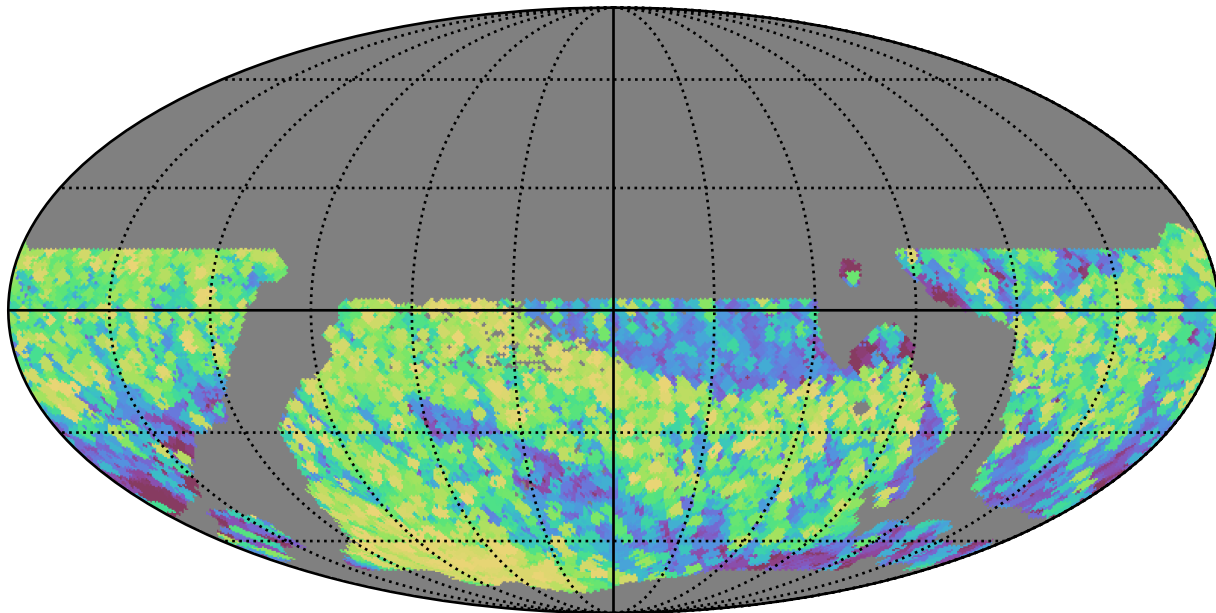
weather_cloudso30v3.4_10yrs WFD all bands: Max airmass
