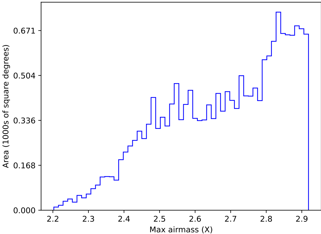
weather_cloudso30v3.4_10yrs WFD all bands: Max airmass
