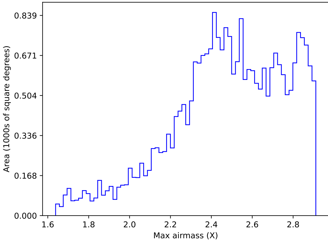
weather_cloudso30v3.4_10yrs All sky z band: Max airmass
