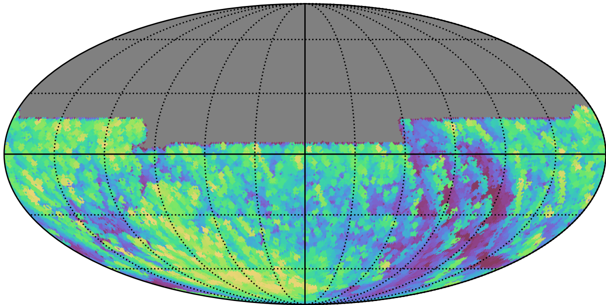
weather_cloudso30v3.4_10yrs All sky y band: Max airmass
