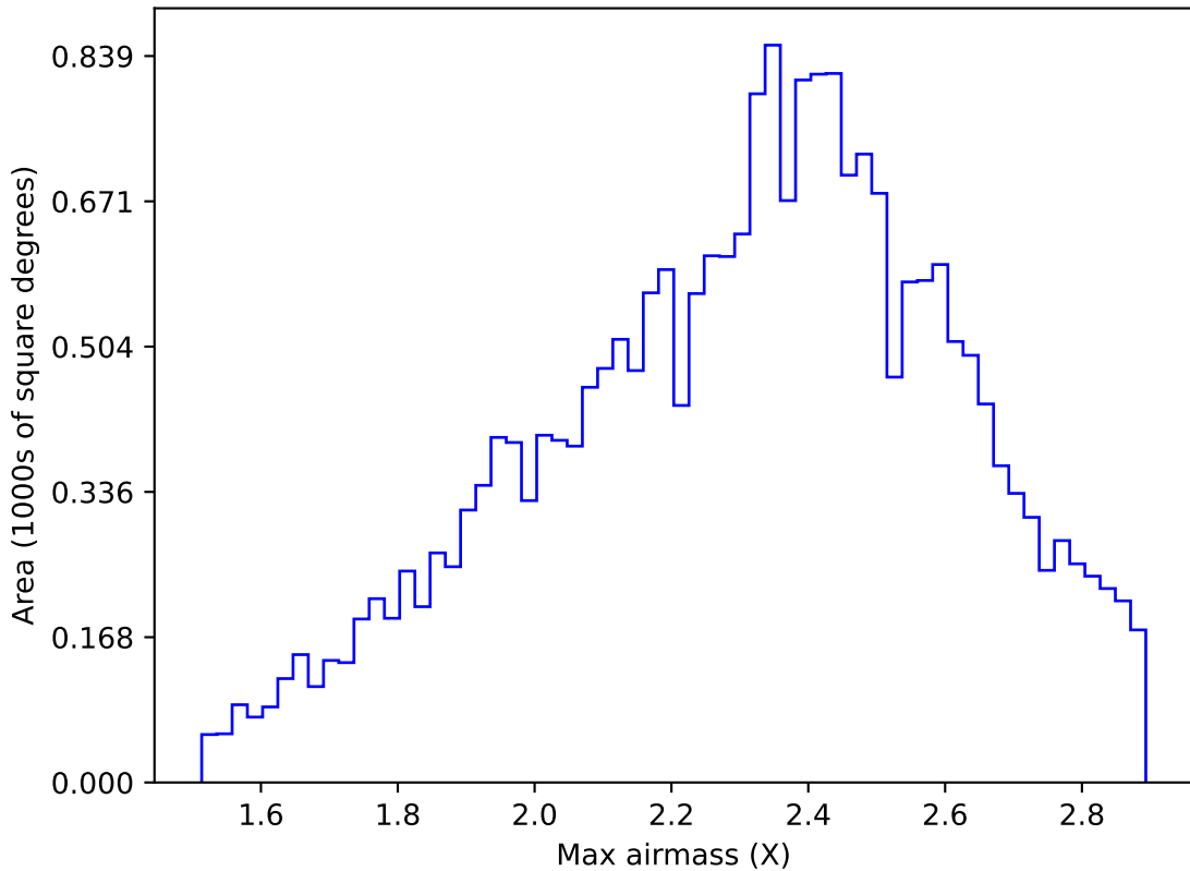
weather_cloudso30v3.4_10yrs All sky y band: Max airmass
