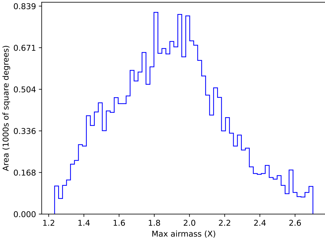
weather_cloudso30v3.4_10yrs All sky u band: Max airmass
