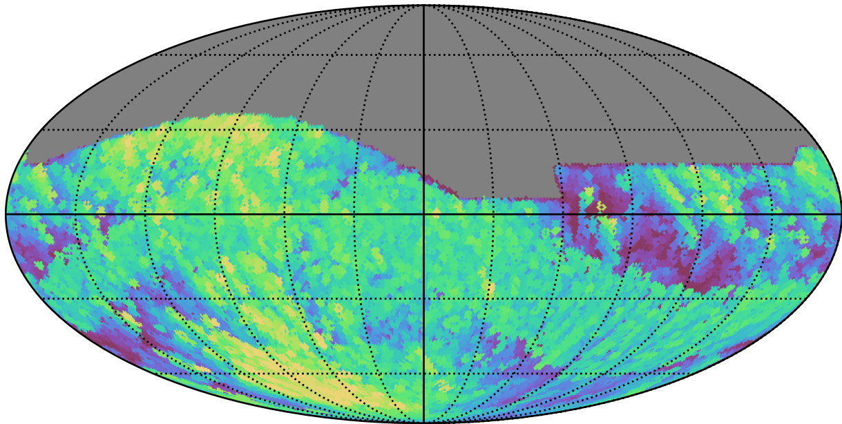
weather_cloudso30v3.4_10yrs All sky r band: Max airmass
