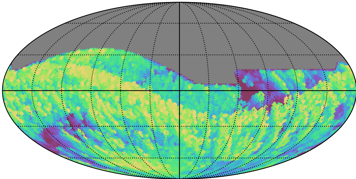
weather_cloudso30v3.4_10yrs All sky i band: Max airmass
