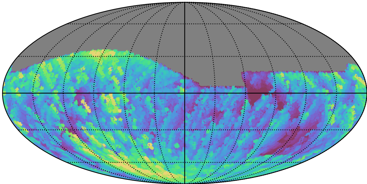
weather_cloudso30v3.4_10yrs All sky g band: Max airmass
