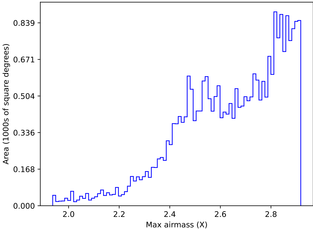
weather_cloudso3v3.4_10yrs All sky all bands: Max airmass
