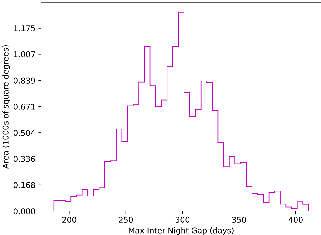
weather_cloudso30v3.4_10yrs WFD z band: Max Inter-Night Gap
