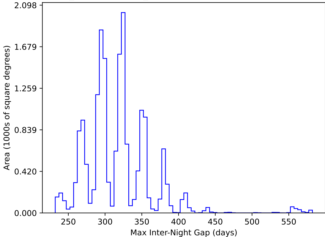
weather_cloudso30v3.4_10yrs WFD y band: Max Inter-Night Gap
