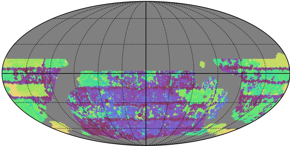
weather_cloudso30v3.4_10yrs WFD u band: Max Inter-Night Gap
