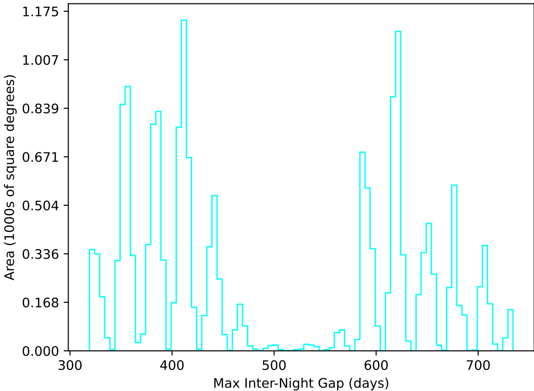
weather_cloudso30v3.4_10yrs WFD u band: Max Inter-Night Gap
