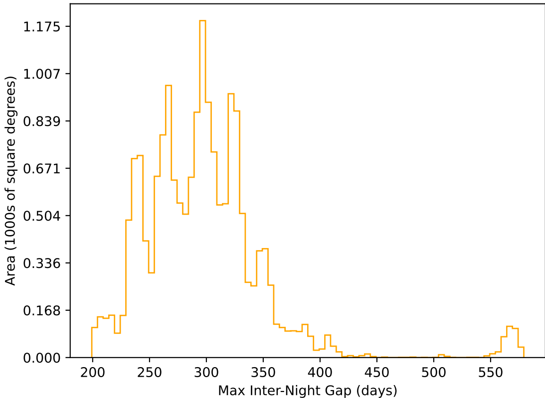
weather_cloudso30v3.4_10yrs WFD r band: Max Inter-Night Gap
