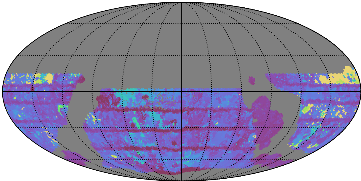
weather_cloudso30v3.4_10yrs WFD i band: Max Inter-Night Gap
