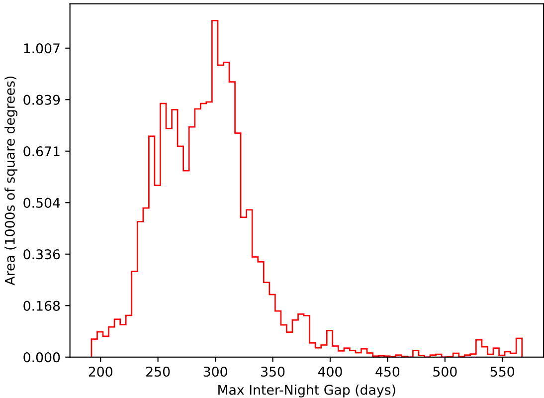
weather_cloudso30v3.4_10yrs WFD i band: Max Inter-Night Gap
