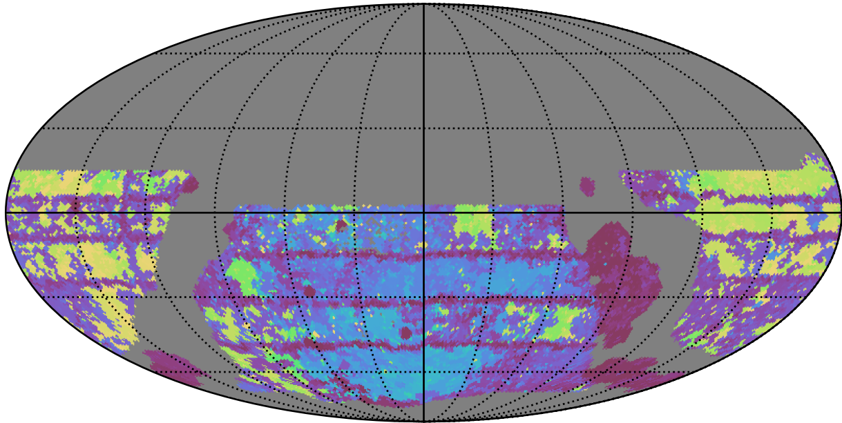
weather_cloudso30v3.4_10yrs WFD g band: Max Inter-Night Gap
