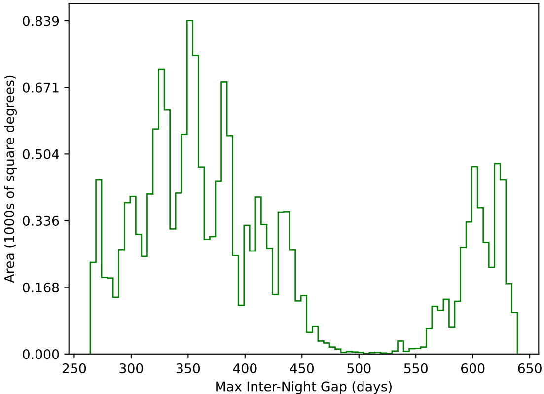
weather_cloudso30v3.4_10yrs WFD g band: Max Inter-Night Gap
