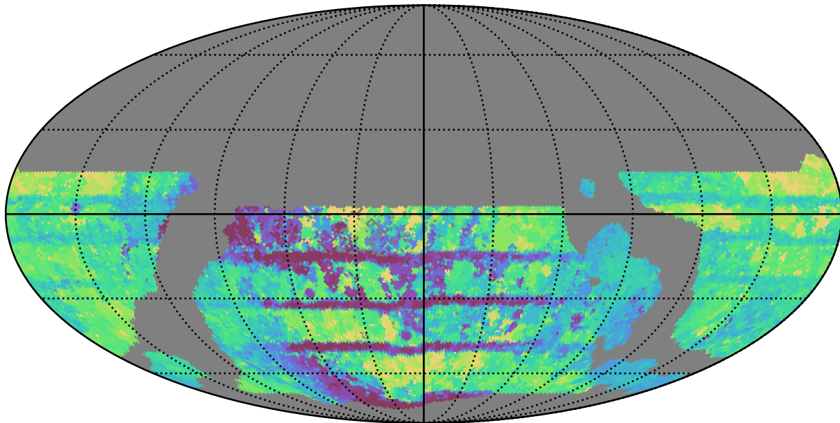
weather_cloudso30v3.4_10yrs WFD all bands: Max Inter-Night Gap
