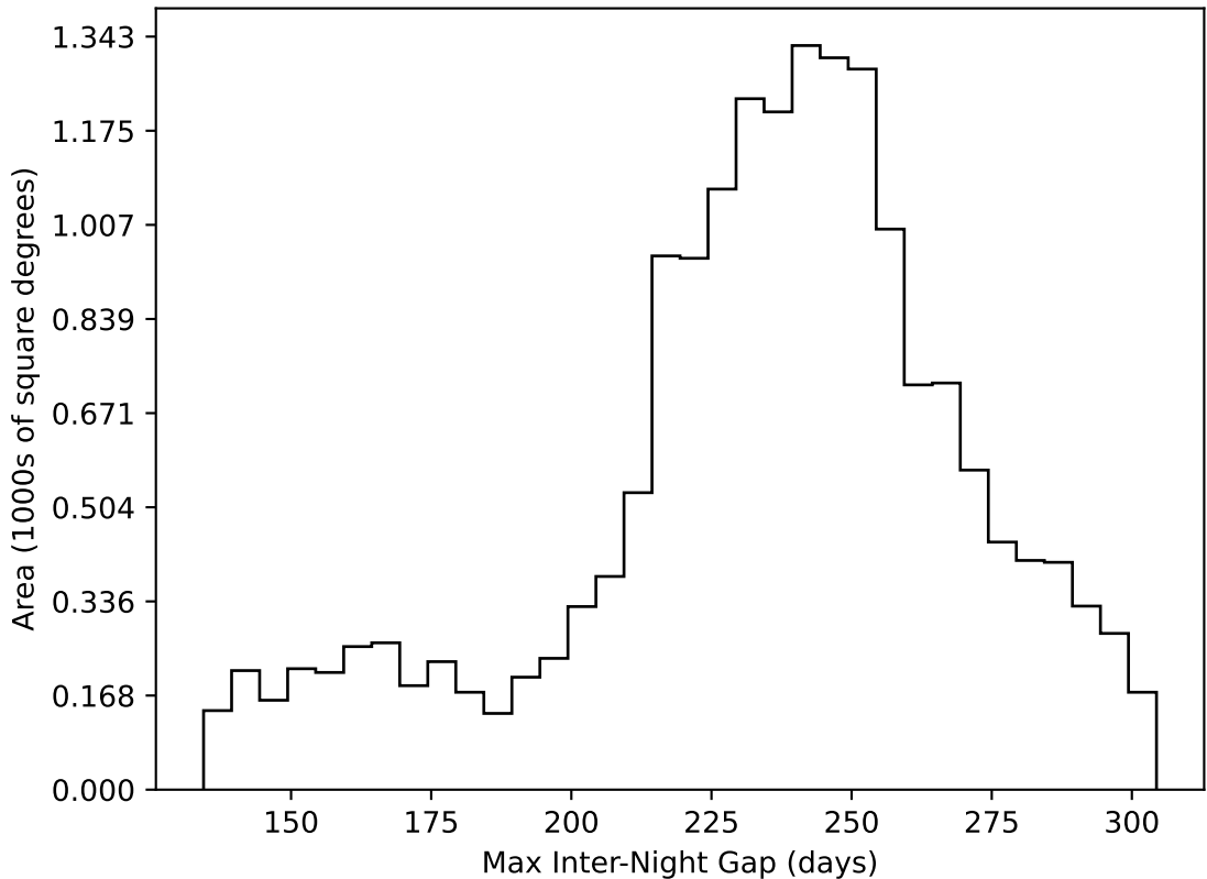
weather_cloudso30v3.4_10yrs WFD all bands: Max Inter-Night Gap
