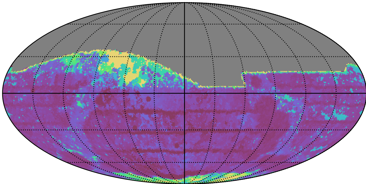
weather_cloudso30v3.4_10yrs All sky z band: Max Inter-Night Gap
