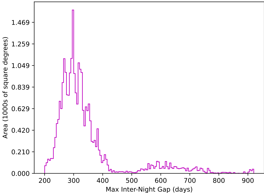
weather_cloudso30v3.4_10yrs All sky z band: Max Inter-Night Gap
