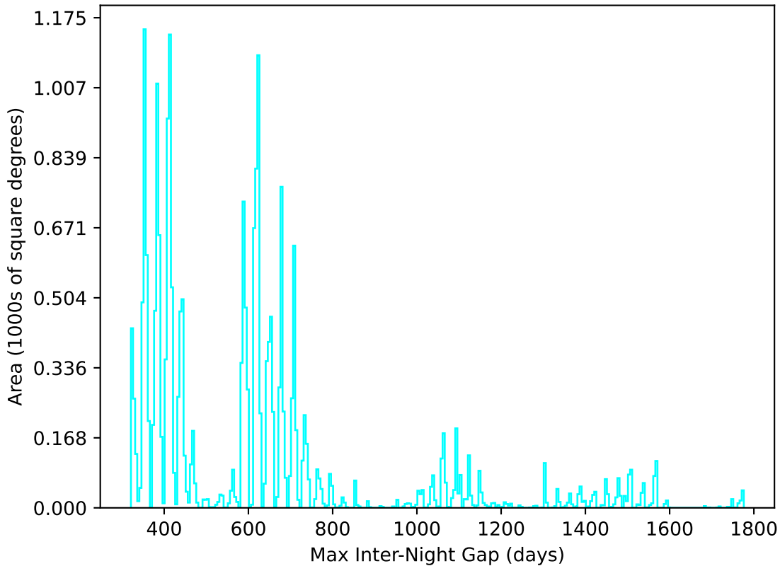
weather_cloudso30v3.4_10yrs All sky u band: Max Inter-Night Gap
